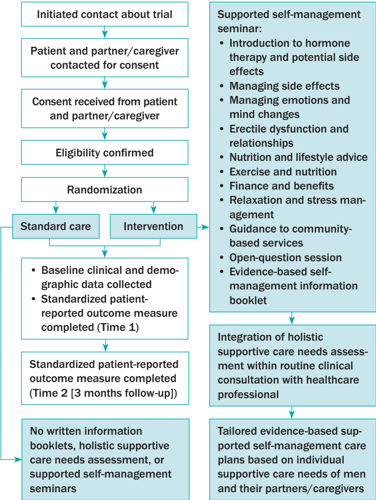
FIGURE 1. Study Overview
